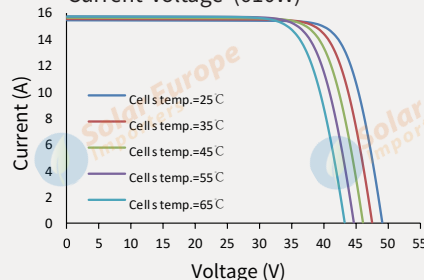
Current-Voltage (610W)
