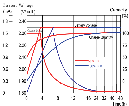
Constant-potential charge
